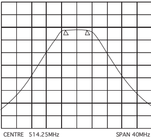
Frequency Response of Input Filter Stages TCFL331, TCFL441, TCFL332, TCFL442 5dB DIV
