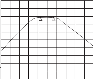
Frequency Response of Input Filter Stages TCFL331, TCFL441, TCFL332, TCFL442 5dB DIV
